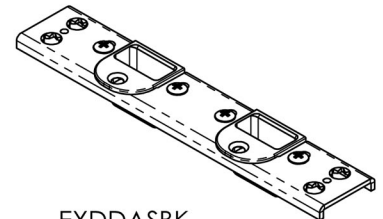
EXDDASBK Double Adjustable Shootbolt Keep (Packers Required)
