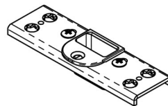
EXDSASBK Single Adjustable Shootbolt Keep (Packers Required)
