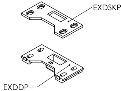
Low Threshold Single Keep
